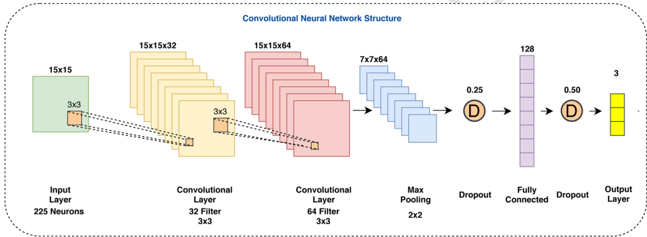
Figure 5: CNN Process
