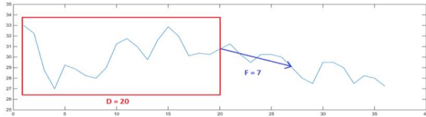
Fig.4. The instance of a sliding window
