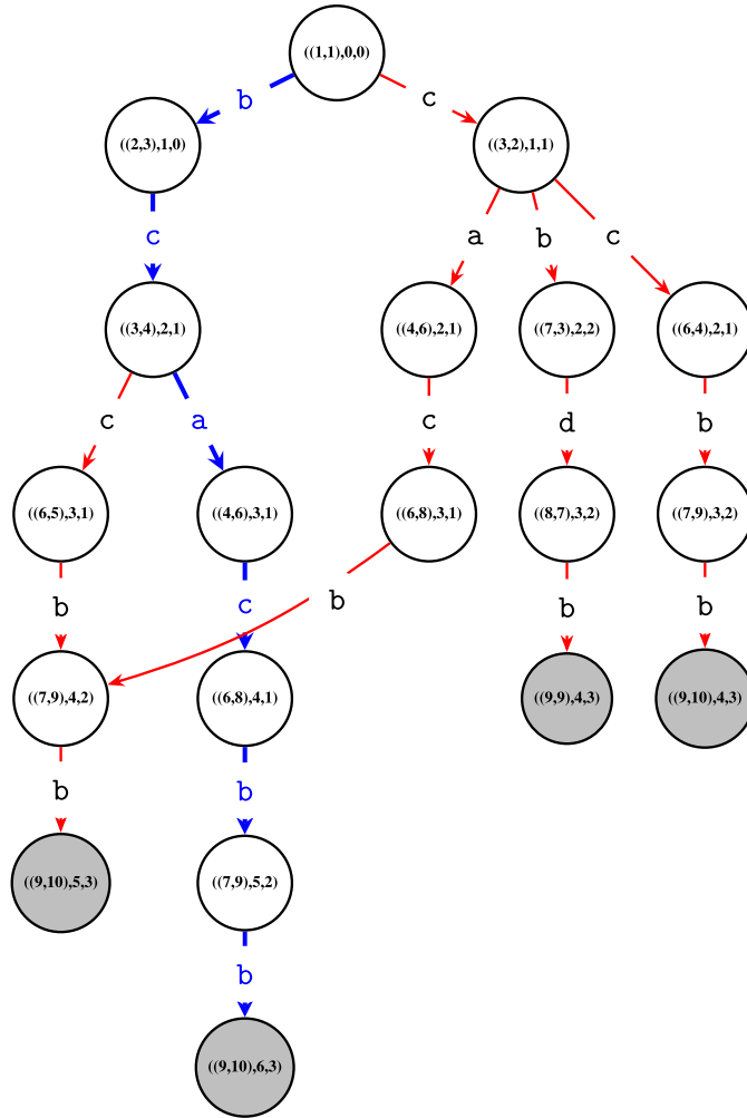
Fig. 1. Example showing the full state graph for the problem instance ( (s_1 = bcaacbdba, s_2 = cbccadcbdd), P = cbb, \Sigma = \{a, b, c, d\} ). There are four sink nodes representing non-extensible solutions (marked by light-gray color). The optimal solution is s = bcacbb of length 6 that corresponds to the node v = (p^v = (9, 10), l^v = 6, u^v = 3) . The longest path that corresponds to the optimal solution is displayed by means of thick arrows.
