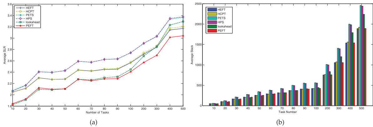
Fig. 3. (a) Average SLR and (b) slack for random graphs as a function of DAG size.
