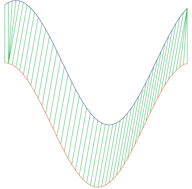
Fig. 1. Two 1D sequences aligned with dynamic time warping. Coordinates of the top and bottom sequences have been, respectively, computed by \cos(t) and \cos(t+\alpha) . For visualization purpose, the top sequence is drawn vertically shifted.
