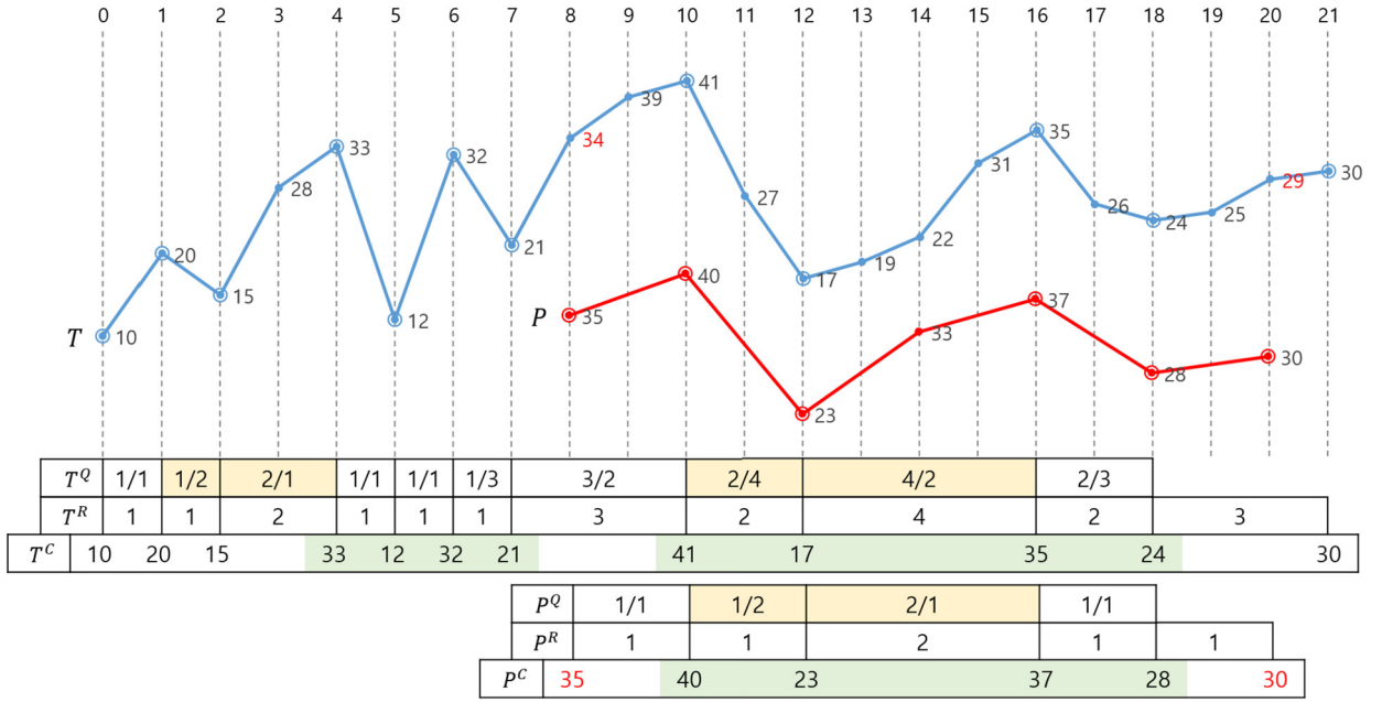
Fig. 2. An example of order-preserving pattern matching with scaling.
