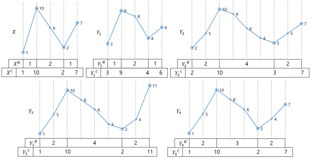
Fig. 1. X^R , X^C , Y_1^R , Y_1^C , Y_2^R , Y_2^C , Y_3^R , Y_3^C , Y_4^R , Y_4^C when the strings X = (1, 10, 6, 2, 7) , Y_1 = (3, 9, 8, 4, 6) , Y_2 = (2, 5, 10, 9, 6, 4, 3, 5, 7) , Y_3 = (1, 5, 10, 8, 6, 3, 2, 4, 11) , and Y_4 = (1, 5, 10, 8, 6, 2, 4, 7) .
