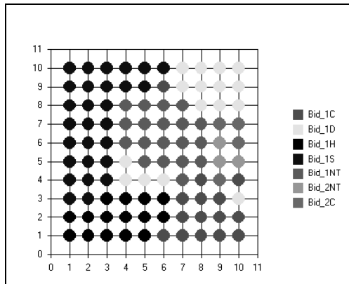
Figure 3: Opening Bids
