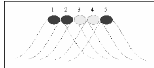
Figure 4: Neighboring Neurons
