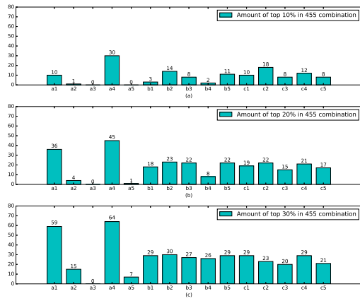
Fig. 2. The appearance amount of each SVM classifier constituting the ensemble classifiers among the 455 combinations, where the x-axis denotes SVM classifiers and y-axis denotes the appearance amount of each SVM classifier. (a) Top 10% accuracies of 455 combinations. (b) Top 20% accuracies of 455 combinations. (c) Top 30% accuracies of 455 combinations.
